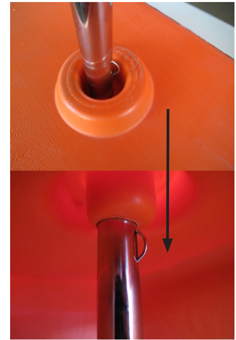
AR Flag with locking push pin and steel dowel.
